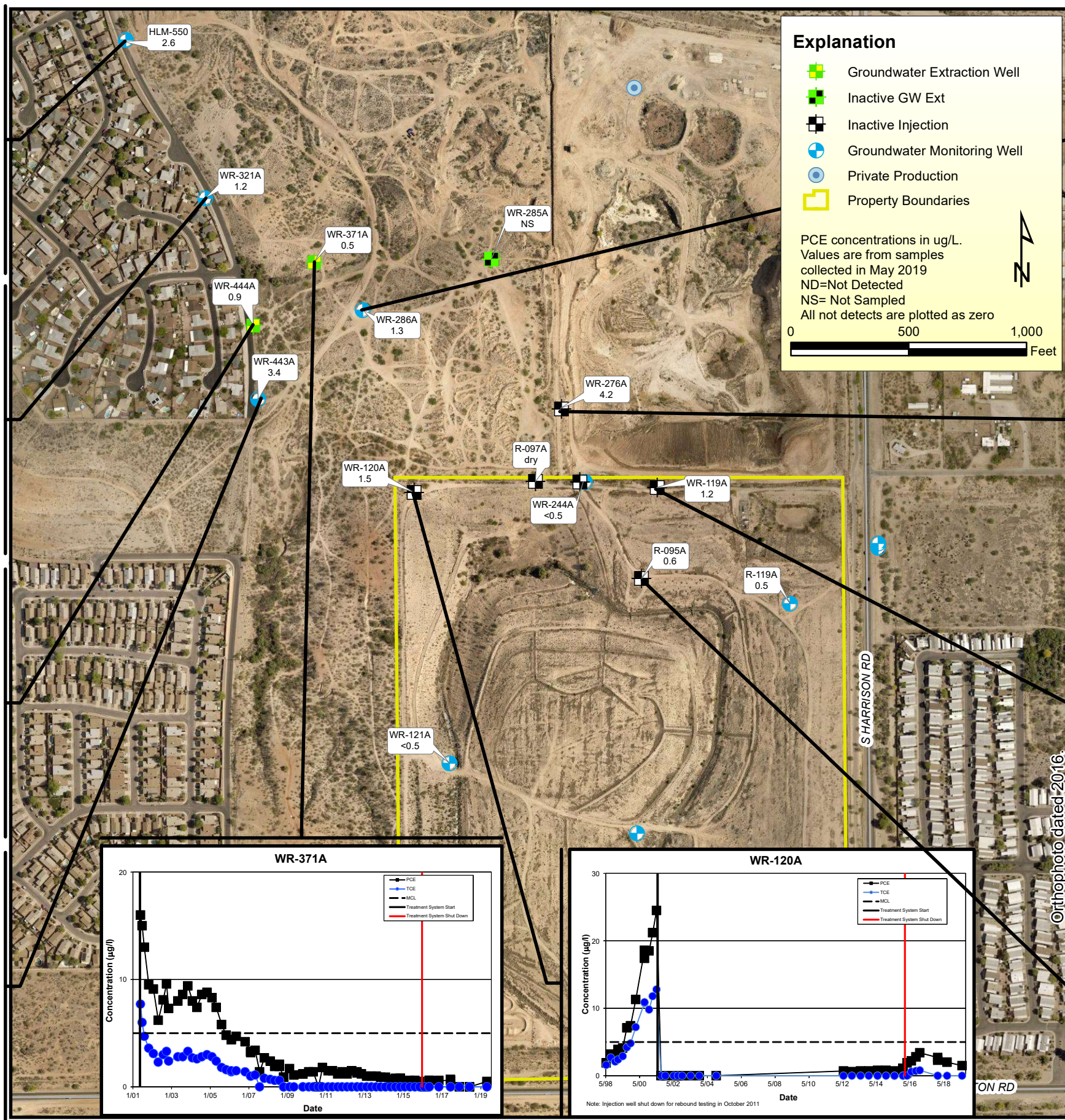
Figure 5 Groundwater TCE and PCE Concentrations - May 2019 Harrison Road Landfill
