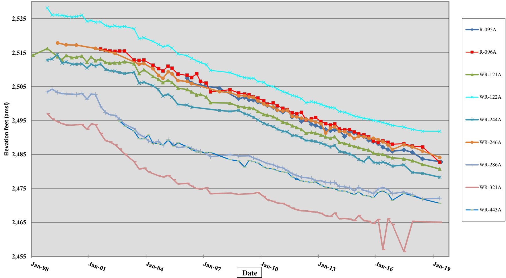
Figure 4 Groundwater Hydrographs Harrison Landfill
