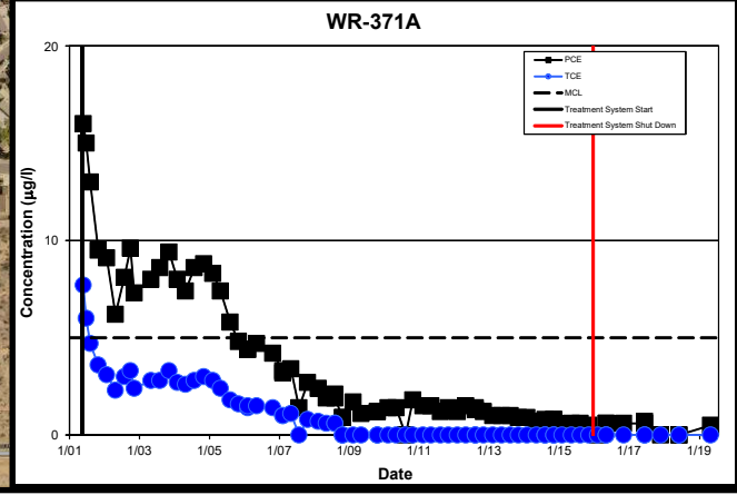
Figure 5 Groundwater TCE and PCE Concentrations - May 2019 Harrison Road Landfill
